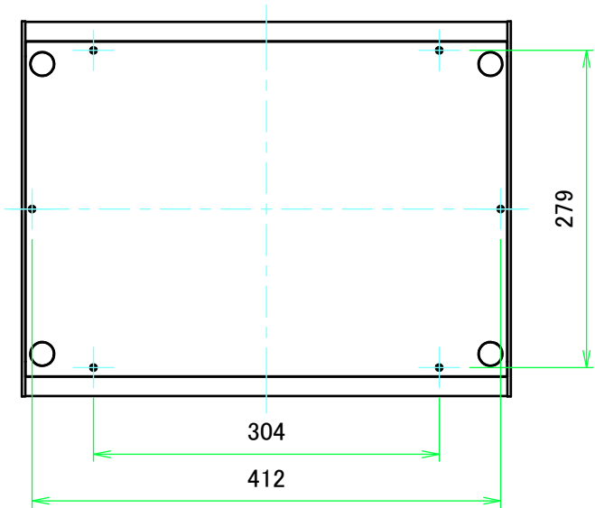
F view
